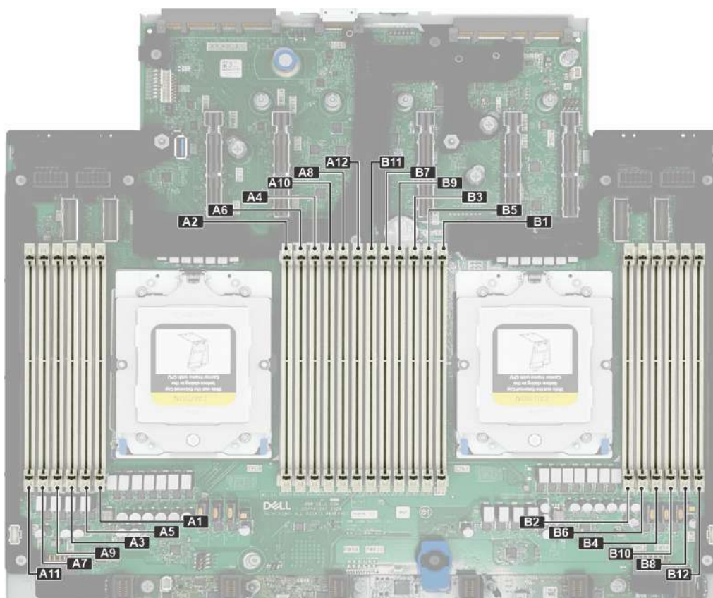
Figure 19. Memory channels
