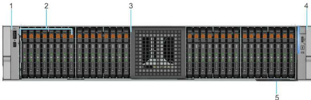
Figure 9. Front view of the 32 x EDSFF E3.S Gen5 NVMe
